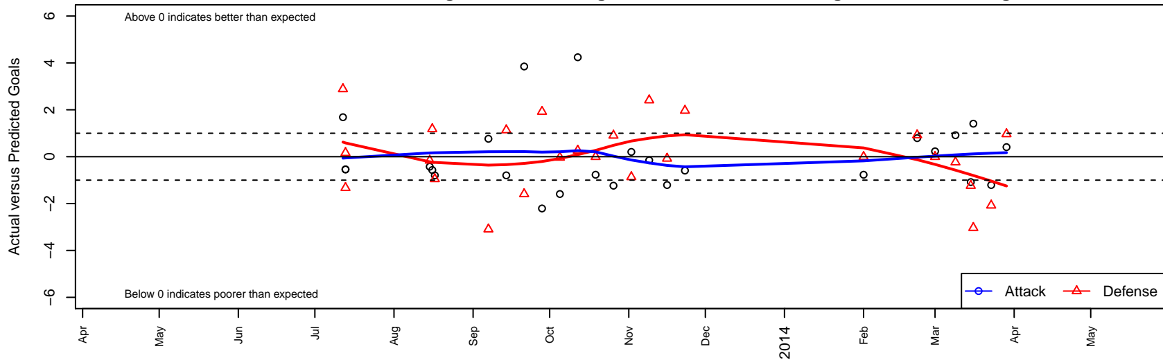
RSA Elite White B00 Dots are actual minus expected GF (blue circles) and GA (red triangles). Blue line is smoothed change in attack strength. Red is smoothed change in defense strength.
